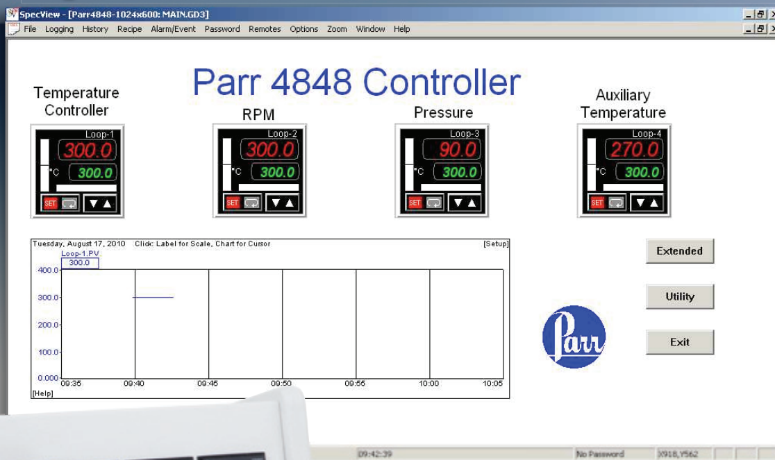
Sample screenshot from a PC running SpecView Software with data from a Parr® 4848 Process Controller.
